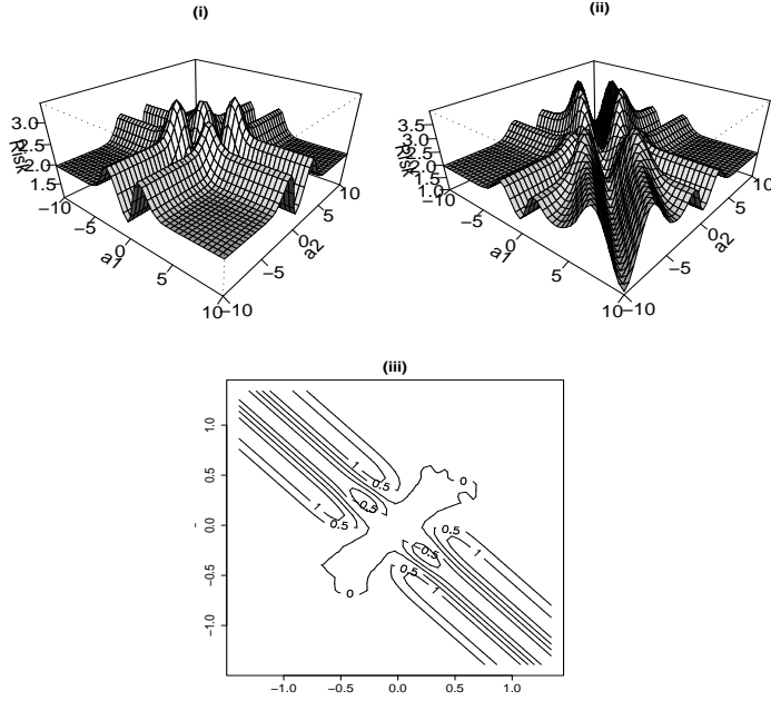
FIGURE 6.1. Limiting mean squared error risk surface \bar{R}(a) using (i) AIC and (ii) FIC for q = 2 , \omega_1 = \omega_2 = 1 and K = \text{diag}(1, 1) . (iii) Risk difference \bar{R}_{\text{fic}}(a) - \bar{R}_{\text{aic}}(a) . The smallest risk for FIC is in the centre stripe and in the two side-lobes.
